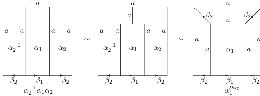
Figure 1. Verification of CM2) for \Pi_2(X, A, a) .
